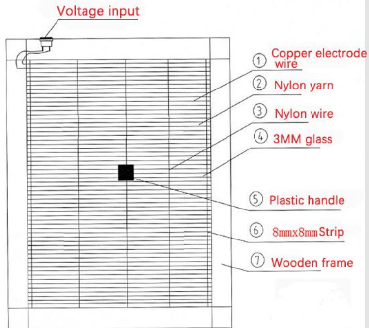
Front view of power grid
