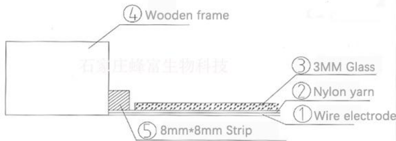
Side view of power grid
